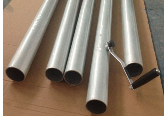
Heavy Duty Alu Tube - Dia 76mm, 2.5mm Thickness
