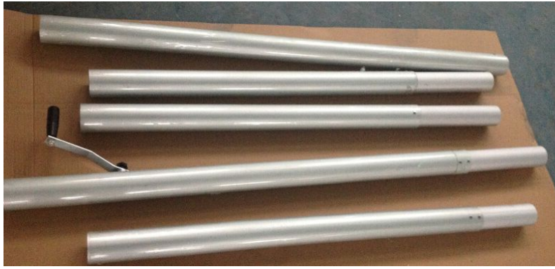
Heavy Duty Alu Tube - Dia 76mm, 2.5mm Thickness
